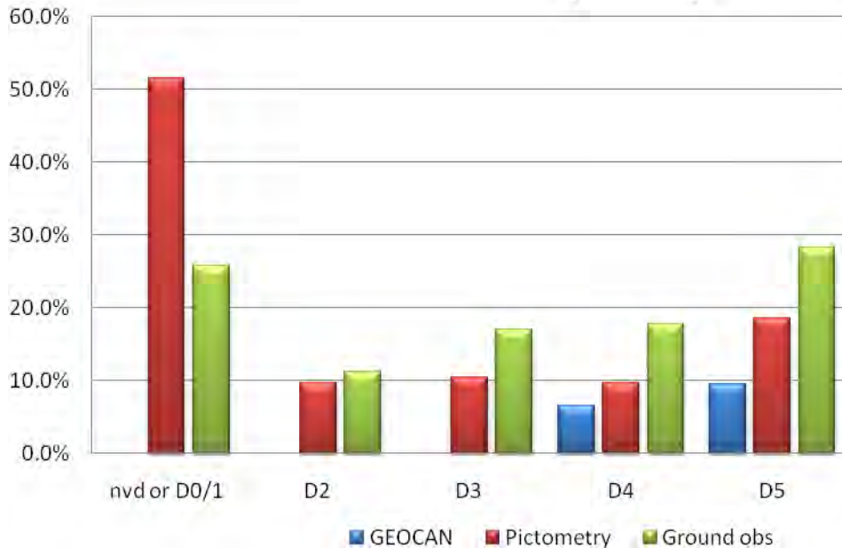
Figure 9. Comparison of GEO-CAN, Pictometry damage assessment and EEFIT ground survey results. N=124.
