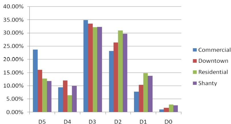
Figure 7 Estimated overall damage distributions assuming binomial distribution governs lower damage levels
