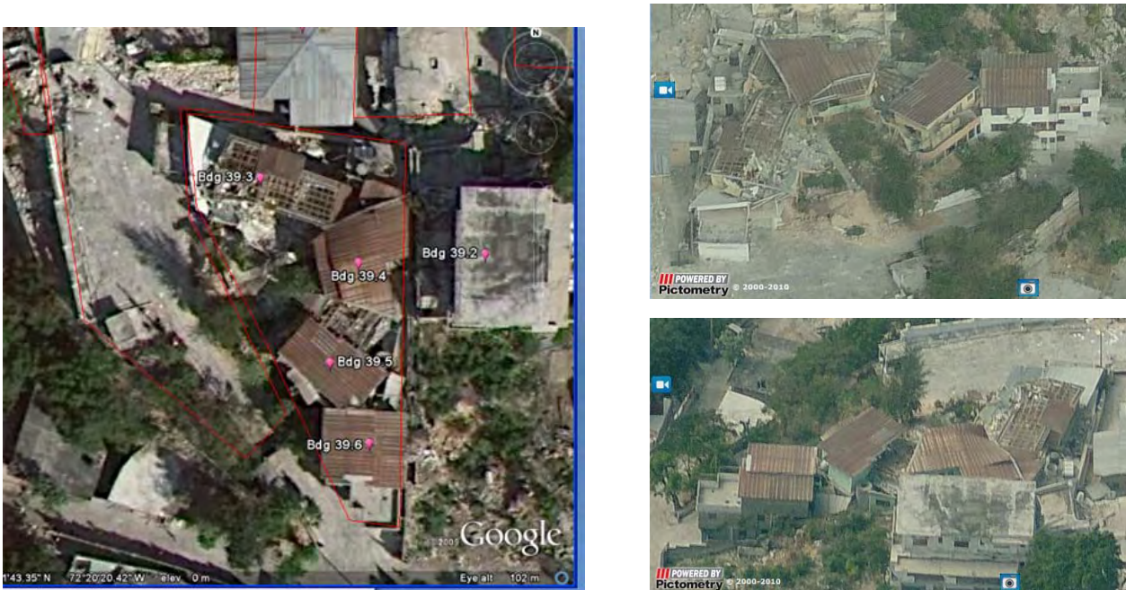
Figure 8 (left) Four Pictometry buildings contained in one GEO-CAN building footprint drawn in red. Pictometry shows that Bdg 39.3 and Bdg 39.4 is one building. (Top right) Same four buildings seen in Pictometry from west to east, (bottom right) same set of buildings seen from east to west. *Note: in the GEO-CAN dataset dated 18 th February 2010, the footprint for this building is smaller, with only Bdg 39.3 delineated as D5. The analysis carried out for this report is based on a GEO-CAN dataset dated 24th February 2010, which is shown in figure 8 above.
