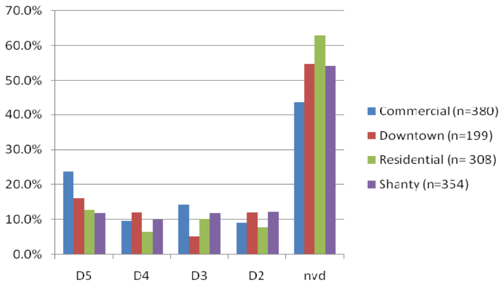
Figure 3. Damage distributions across 1241 buildings in PaP urban area from Pictometry survey, divided by land-use class.
